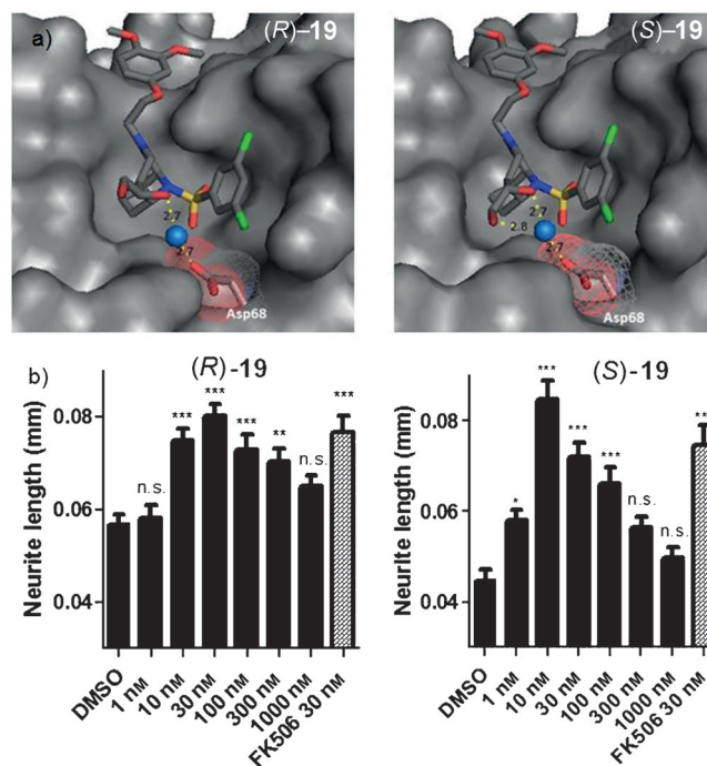
Figure 2. a) Cocrystal structures of ( R )- 19 (PDB: 4W9O) and ( S )- 19 (PDB: 4W9P) in complex with the FK506-binding domain of FKBP51. Hydrogen bonds are indicated by yellow dotted lines with distances in Å. The conserved water molecule is shown as a blue sphere and the van der Waals surface of the interacting Asp68 is shown as wire mesh. b) Stimulation of neurite outgrowth by ( R )- 19 and ( S )- 19 . N2a cells were transfected with a plasmid encoding a myristoylated yellow fluorescent protein, deprived of serum, and treated with the compounds for 24 h, followed by fluorescence imaging and morphological analysis. FK506 at its most effective concentration (30 nM) was included as a positive control. Data represent averages of more than 35 cells. Error bars represent \pm standard error. ***: p < 0.001 , **: p < 0.01 , *: p < 0.05 , n.s.: not significant.
