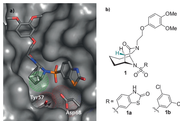
Figure 1. a) Cocystal structure of 1a in complex with the FK506-binding domain of FKBP51 (PDB code: 4JFK, from Ref. [6a]). The free space for a pro-(S)-C 5 substituent is shown as green wire mesh. Residues in close proximity to a potential pro-(S)-C 5 substituent (Tyr57 and Asp68) are shown as sticks and wire mesh. b) Examples of C 5 -unsubstituted [4.3.1] bicyclic FKBP ligands. [6] The pro-(S)-C 5 position is indicated in green.
