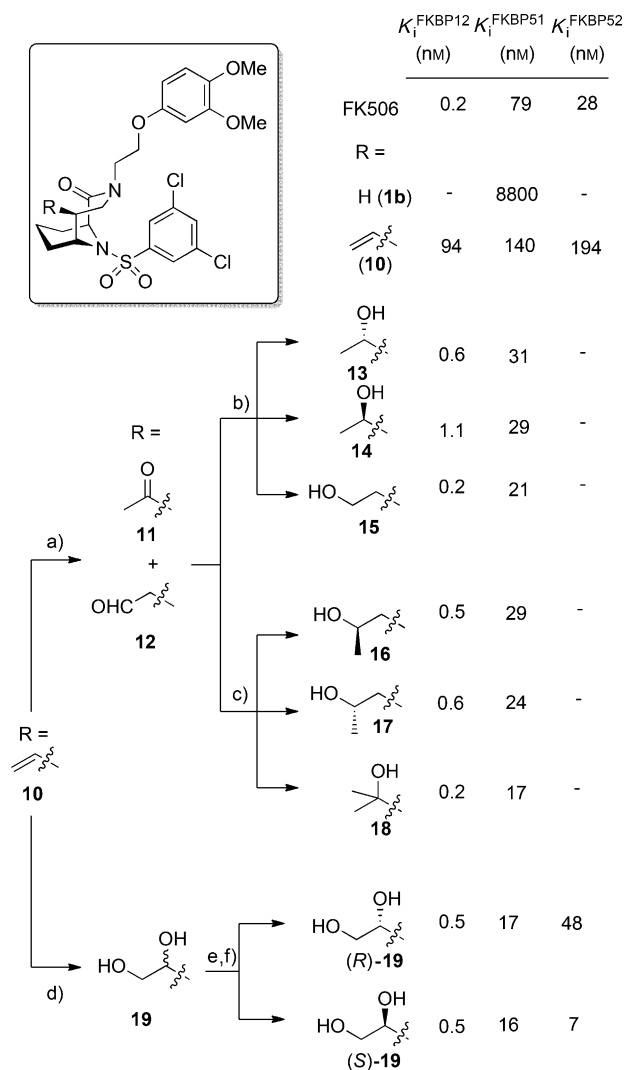
Scheme 3. Reagents and conditions: a) \text{PdCl}_2 , \text{CuCl} , \text{O}_2 , \text{DMF}/\text{H}_2\text{O} , RT, 24 h. b) 1. \text{NaBH}_4 , \text{EtOH}/\text{CH}_2\text{Cl}_2 , RT, 1 h; 13 : 16%, 14 : 9%; 15 : 23% (over 2 steps each). c) \text{MeMgBr} , THF, -78^\circ\text{C} , 1 h; 16 : 12%; 17 : 9%; 18 : 34% (over 2 steps each). d) AD-Mix- \beta , t\text{BuOH}/\text{H}_2\text{O} , RT, 24 h, 75%. e) TBDMSOTf, 2,6-Lutidine, \text{CH}_2\text{Cl}_2 , 1 h, preparative HPLC. f) TBAF, THF, RT, 30 min. Binding to FKBP12 or the FK506-binding domain of FKBP51 or FKBP52 was determined by a competitive fluorescence polarization assay with 40-fluorescein-Gly-rapamycin as a tracer. [11] DMF = N,N -dimethylformamide, TBAF = tetra- n -butylammonium fluoride, TBDMS = tert -butyldimethylsilyl, Tf = trifluoromethanesulfonyl.
