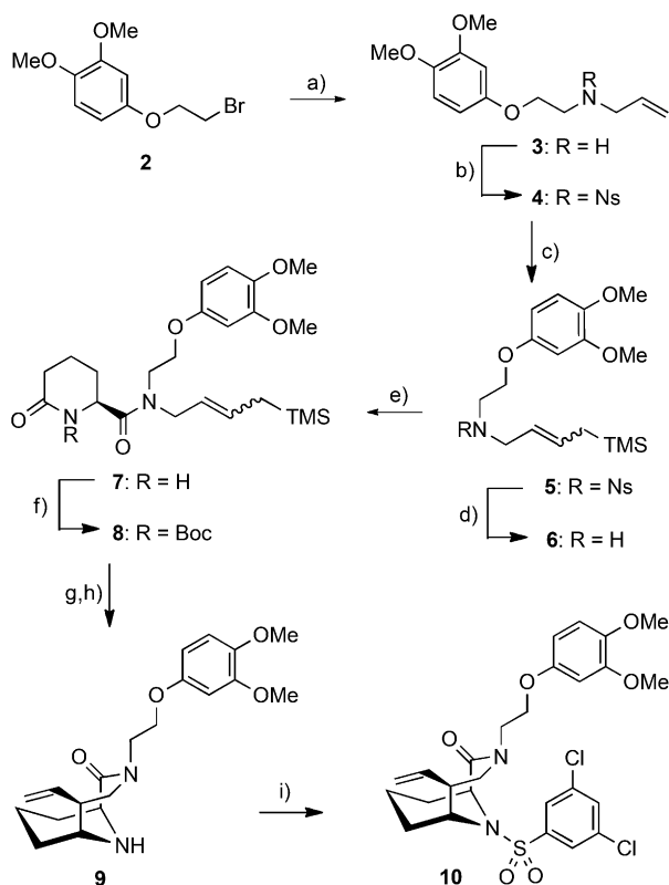
Scheme 2. Reagents and conditions: a) Allylamine, \text{CH}_2\text{Cl}_2 , 50 °C, 24 h, 85 %. b) NsCl, TEA, \text{CH}_2\text{Cl}_2 , RT, 1 h, 95 %. c) AllylTMS, p -benzoquinone, Grubbs-Hoveyda II gen, \text{CH}_2\text{Cl}_2 , 60 °C, 2 h, 95 %. d) PhSH, \text{K}_2\text{CO}_3 , DMF, RT, 2 h, 65 %. e) (S)-6-Oxo-2-piperidinecarboxylic acid, HATU, DIPEA, DMF, RT, 2 h, 72 %. f) \text{Boc}_2\text{O} , TEA, DMAP, \text{CH}_2\text{Cl}_2 , RT, 3 h, 86 %. g) DIBAL-H, THF, –78 °C. h) HF-Pyridine, \text{CH}_2\text{Cl}_2 , –78 → 0 °C, 1 h, 55 % (2 steps). i) 3,5-Dichlorobenzenesulfonyl chloride, DMAP, DIPEA, \text{CH}_2\text{Cl}_2 , RT, 24 h, 55 %. DIBAL-H = diisobutylaluminum hydride, DIPEA = N,N -diisopropylethylamine, DMAP = 4-dimethylaminopyridine, HATU = O-(7-azabenzotriazol-1-yl)- N,N,N' , N' -tetramethyluronium hexafluorophosphate, NsCl = 2-nitrobenzenesulfonyl chloride, TEA = triethylamine, THF = tetrahydrofuran, TMS = trimethylsilane.
